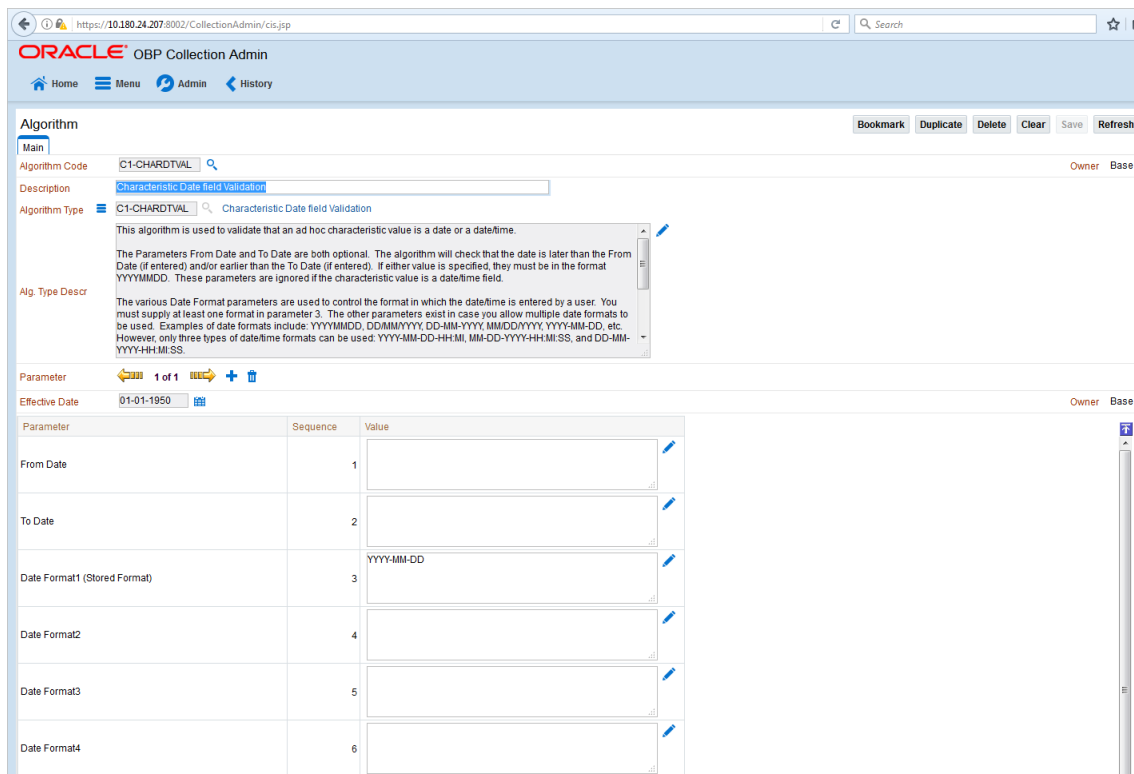
Figure 19–13 Attach Algorithm
